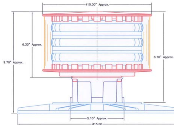
L-864LED Beacon Light
